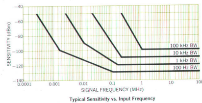
Typical Sensitivity vs. Input Frequency
